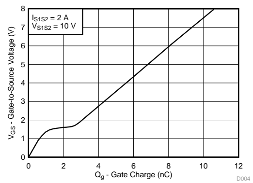
栅极电荷
