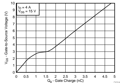
栅极电荷
