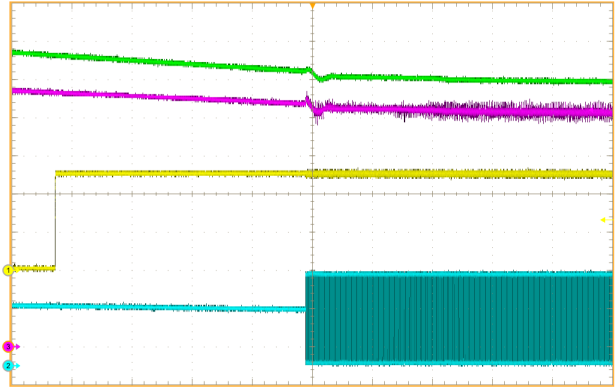
Figure 30. OVP1 Release at V_{\text{FB}} \leq 110\% V_{\text{REF}}
