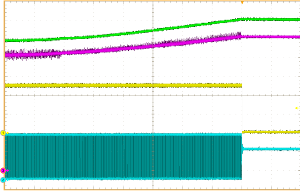
Figure 29. OVP1 at V_{\text{FB}} \geq 115\% V_{\text{REF}}
