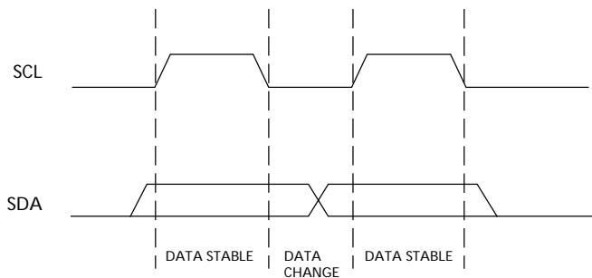
Figure 15: Data Validity
