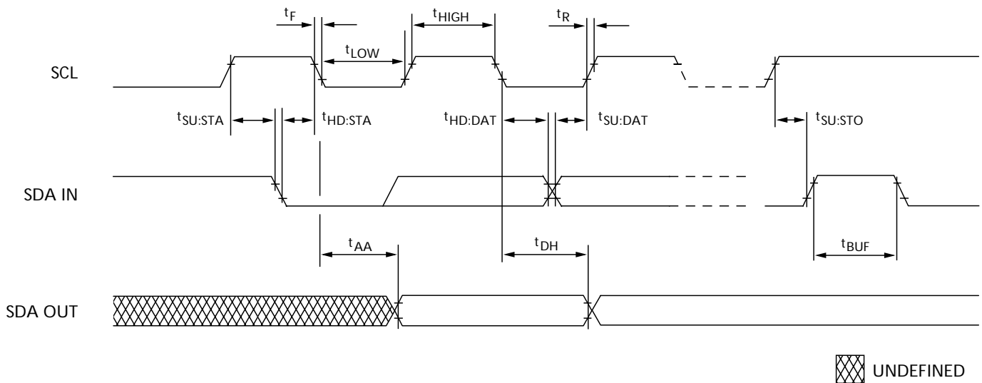
Figure 18: SPD EEPROM Timing Diagram
