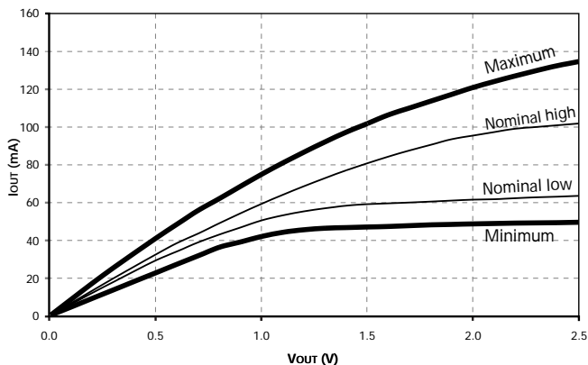
Figure 11: Pull-Down Characteristics
