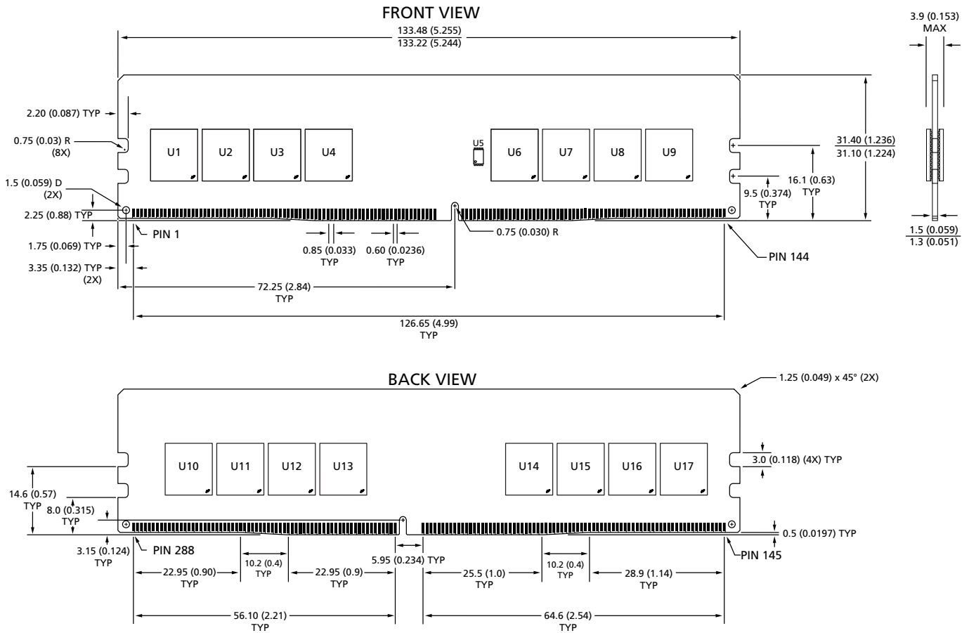
Figure 5: 288-Pin DDR4 UDIMM (R/C B2)
