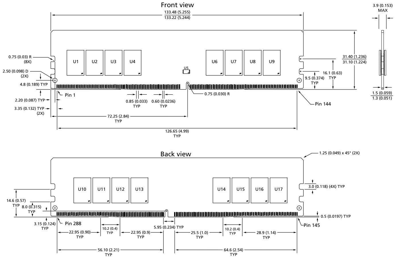
Figure 4: 288-Pin DDR4 UDIMM (R/C B1)
