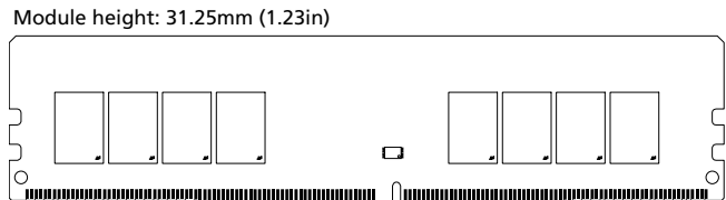
Figure 2: 288-Pin UDIMM (R/C-B2)
