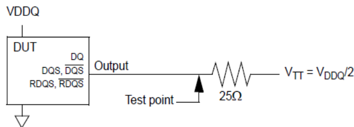
Slew rate test load
