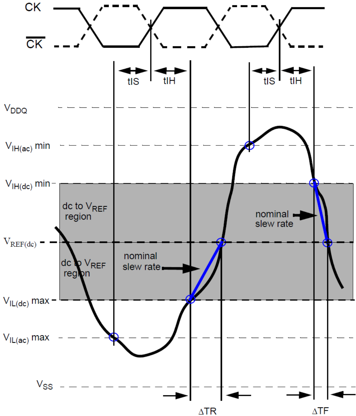
Illustration of nominal slew rate for t IH
