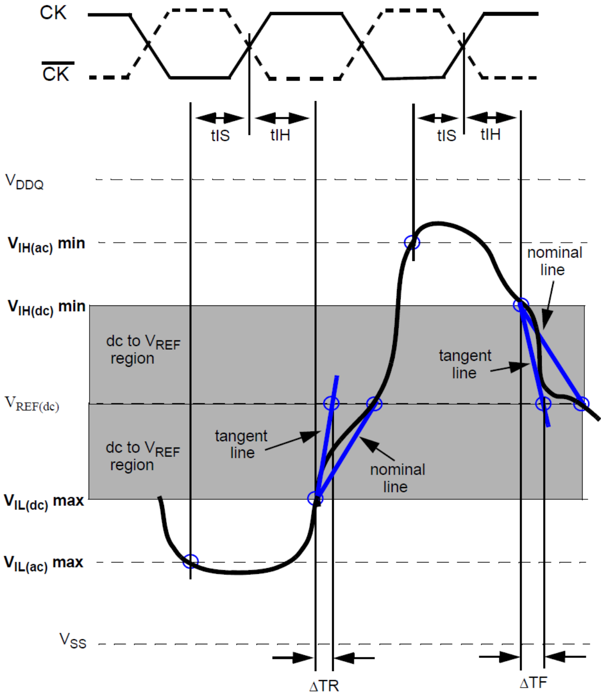
Illustration tangent line for tIH
