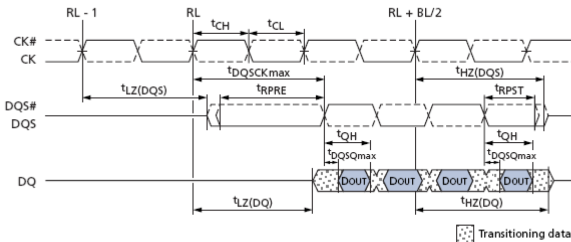
Data output (Read) timing ( t_{DQSQmax} )
