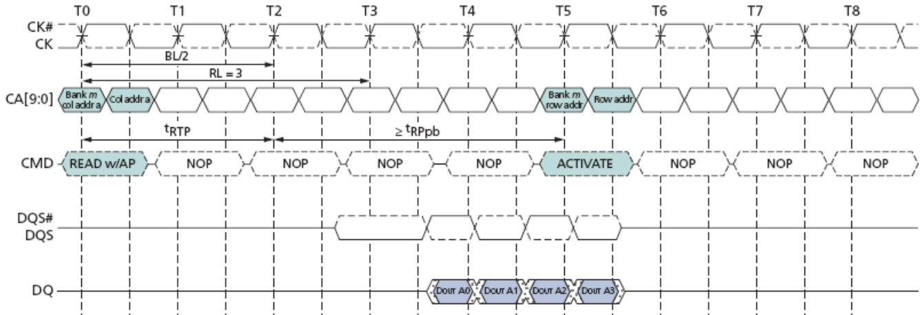
Burst Read with Auto-Precharge: RL=3, BL=4, RU( t_{RTP}(\min)/CK )=2
