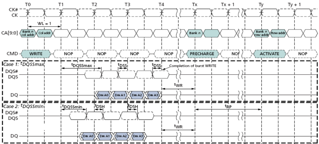
Data input (Write) timing
